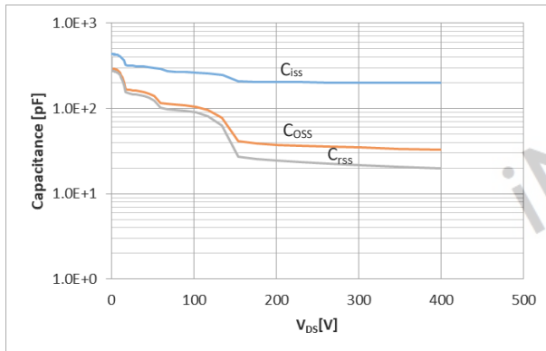
Figure 5. Typical Capacitance
