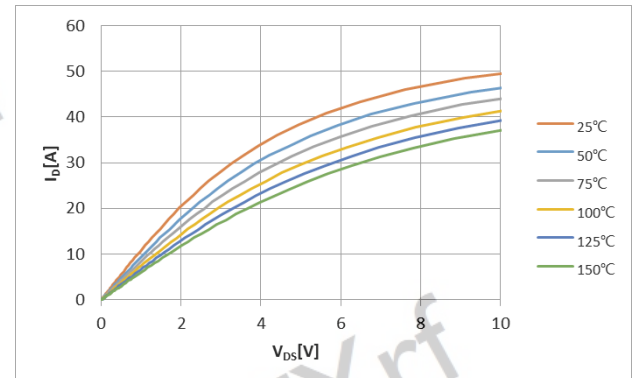
Figure 8. Characteristics for various temperatures Parameter: T_J
