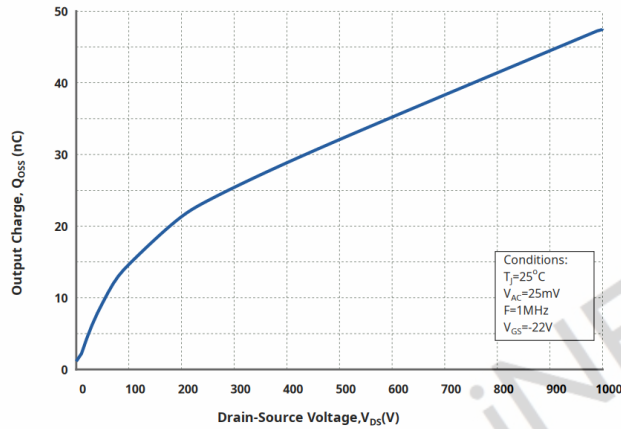
Figure 9. Typical output charge Q_{oss}
