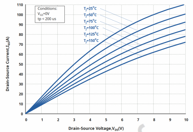
Figure 8. Characteristics for various temperatures Parameter: T_J
