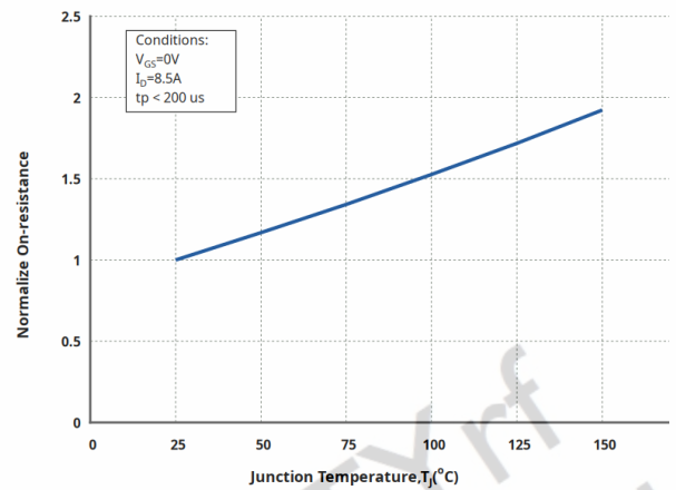
Figure 4. Normalized On-resistance I_D = 8.5\text{ A} , V_{GS} = 10\text{ V}
